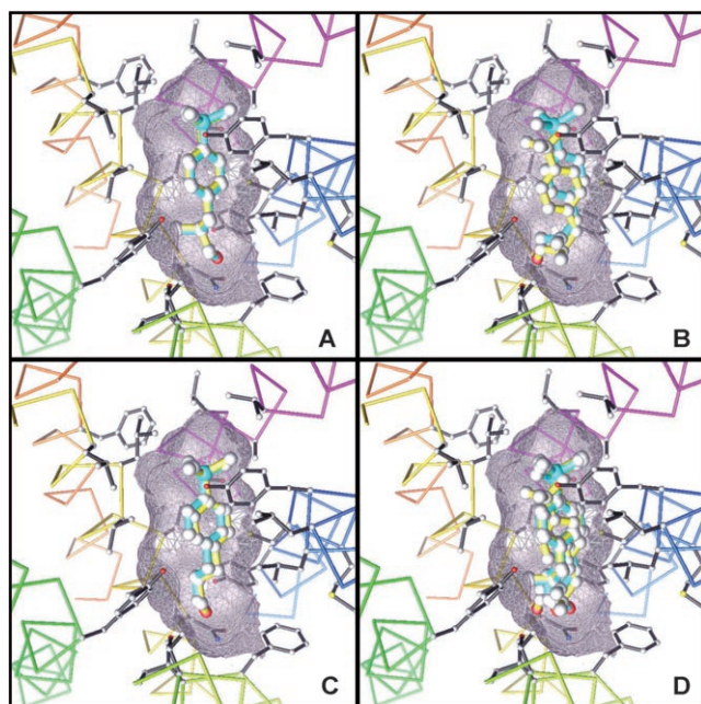
Figure 1. Docking of A) (S)-lilial [(S)-1a], B) (R)-lilial [(R)-1a], C) bourgeonal (2a) (all shown in yellow) and their respective silicon analogues (S)-1b, (R)-1b, and 2b (cyan) on the calculated hOR17-4 receptor model, and D) superposition of all ligands.
