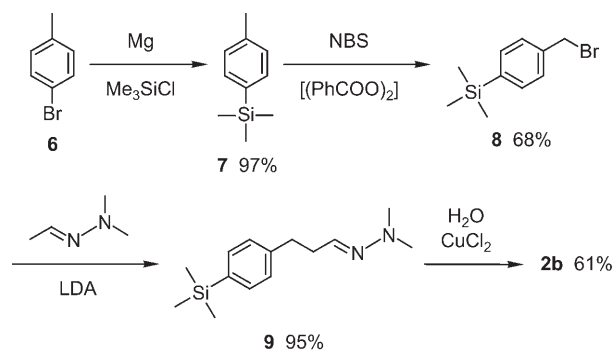
Scheme 3. Synthesis of sila-bourgeonal (2b).
