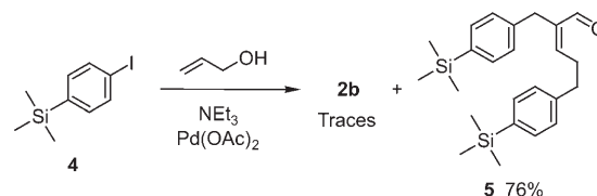
Scheme 2. Reaction of 4 with prop-2-en-1-ol.
